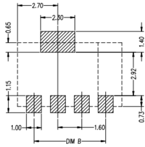
3&4PIN LAYOUT 5-10PIN LAYOUT RECOMMENDED PCB LAYOUT TOL:(±0.05)
