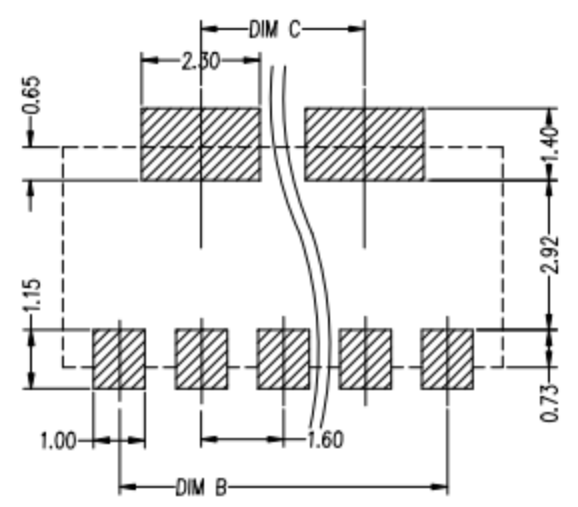
3&4PIN LAYOUT 5-10PIN LAYOUT RECOMMENDED PCB LAYOUT TOL:(±0.05)
